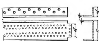
Figs. 3752-3755. Stop Channel.
